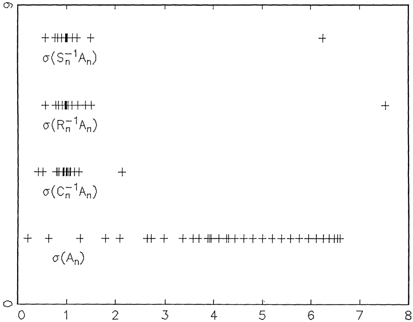
FIGURE 1 Spectra of the preconditioned systems for n = 32
